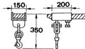
MINF-1 Used with one fork
