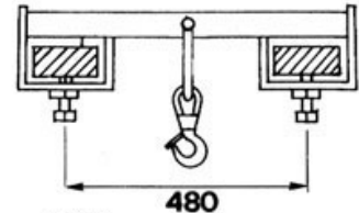
MINF-2 Used with two forks
